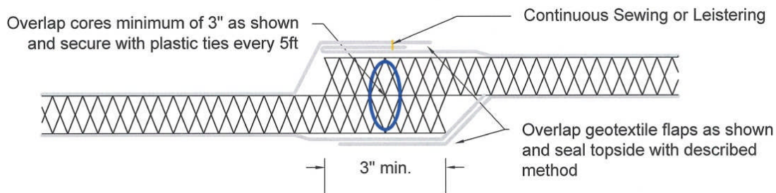
Figure 1. Overlap along roll length
